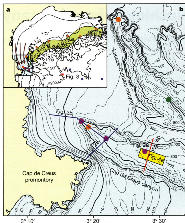
Figure 1 | Bathymetry maps and station location. a , Bathymetry map of Gulf of Lions (GL). Mooring stations shown as orange dots, for 2003–04 at 300 m; purple, winter 2004–05 at 200, 500 and 750 m; and green, long term mooring at 1,000 m. Deep hydrological stations at (red square) and off (blue square) the mouth of the Cap de Creus Canyon (CCC) are also shown (see Fig. 3). Arrows indicate the direction of the mean coastal (brown) and slope circulation (green). b , Detailed bathymetry of the southwestern end of the GL. Time series shown in Fig. 2a correspond to the 750 m mooring (purple dot) inside CCC. Locations of the hydrological sections in Fig. 3 (blue lines), and of the side scan sonar sonograph (yellow box) and section line (red line) in Fig. 4 are also indicated.
