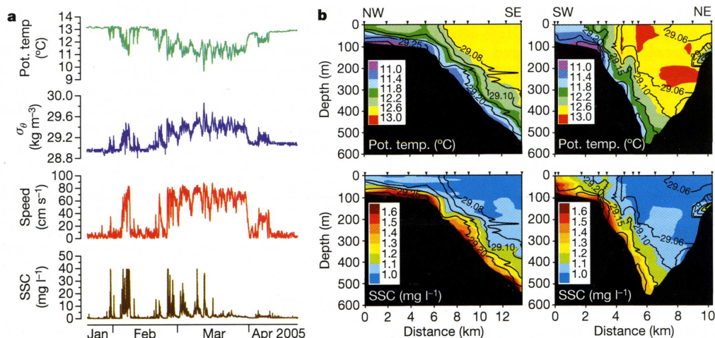
Figure 2 | Time series and sections of key parameters in the CCC. a, Potential temperature, potential density anomaly, current speed and suspended sediment concentration records at 750 m depth during the cascading period of winter 2004–05. DSWC events correspond to temperature drops concomitant with density increases. b, Potential temperature and suspended sediment concentration sections with potential
