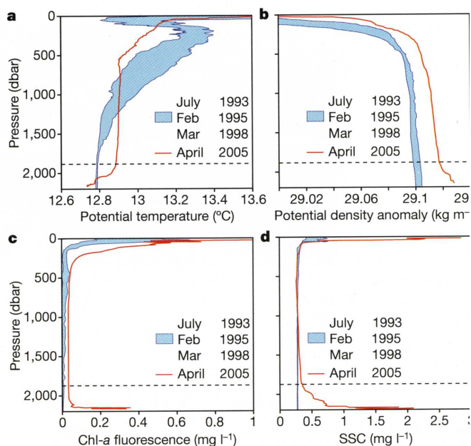
Figure 3 | Deep comparative profiles of key parameters at and off the C mouth. a, Potential temperature. b, Potential density anomaly.
